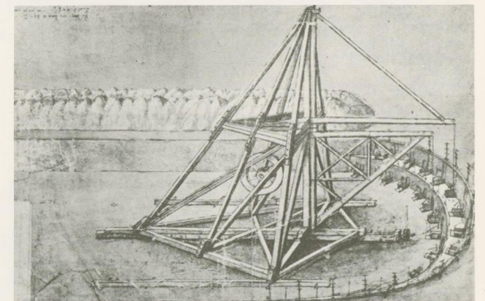
▲ Double crane for construction of canals Ambrosian Library, Milan
